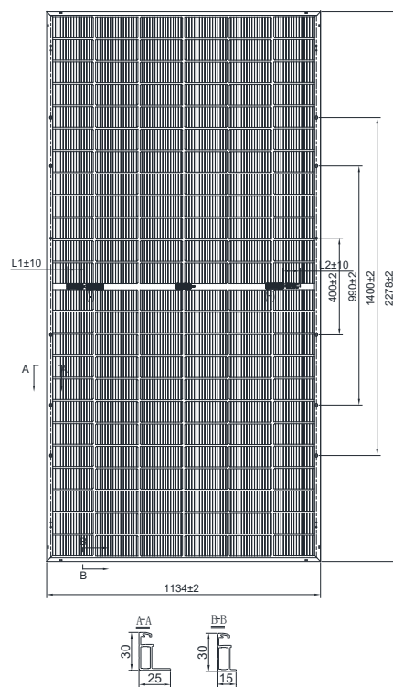
Aluminum Frame
